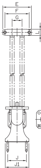
DIMENSIONS - mm
