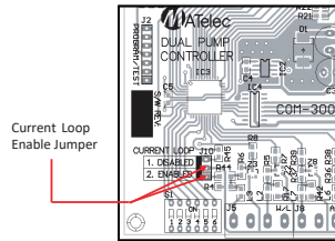
Figure 1: APCB PCB Layout and Current Loop Jumper
