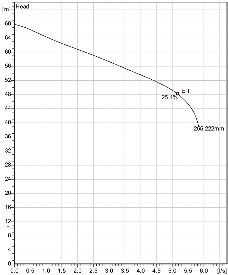
Curve according to: ISO 9906
