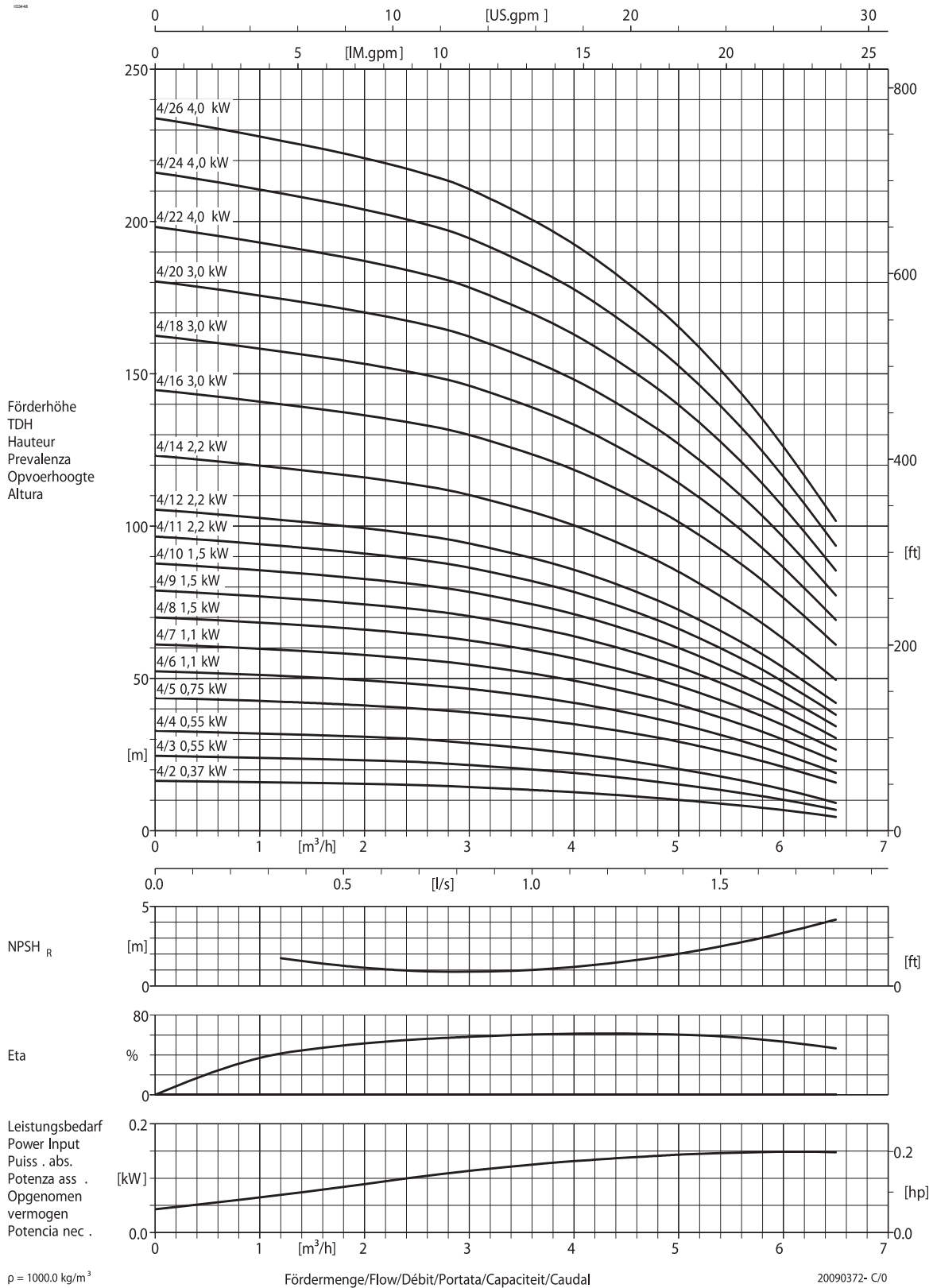
Performance curve V(C/S) B - 50Hz - 2 pole
