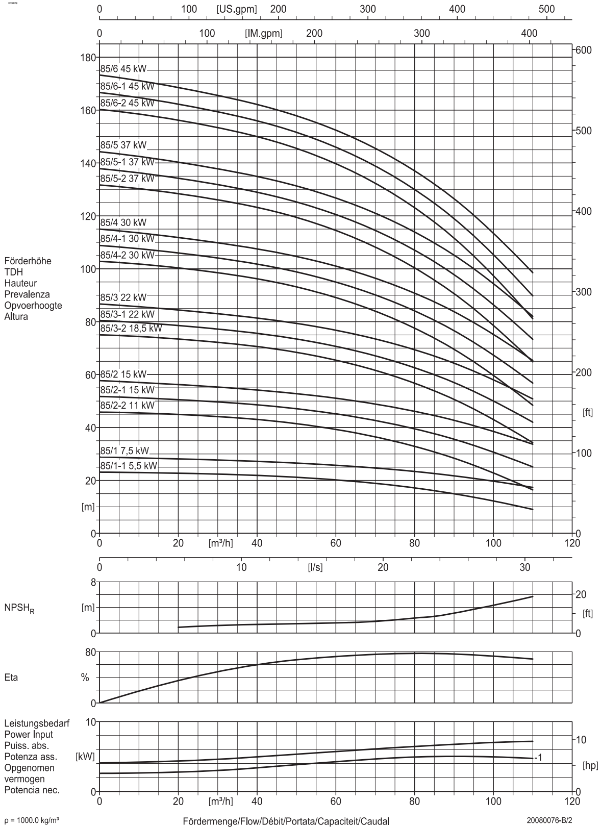
Performance curve V(C/S) 85 B - 50Hz - 2 pole
