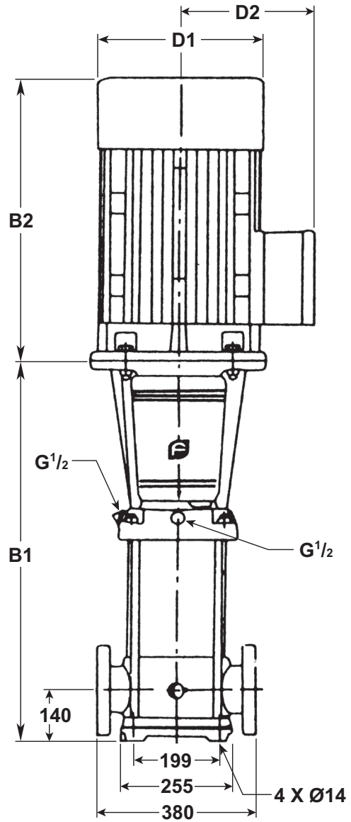
VM90 – PN16
