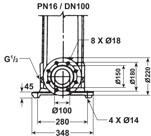
VM90 – PN16
