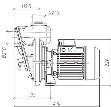
EASM (3Φ)
