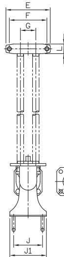
DIMENSIONS - UMDNSS5500/80/3
