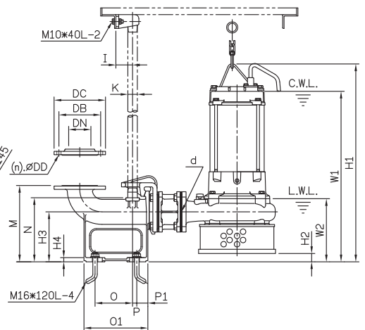
DIMENSIONS - UMDNSS5500/80/3
