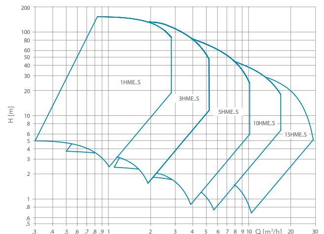
Performance curve, e-HM smart
