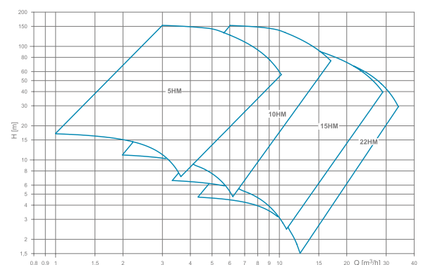
Performance curve, e-HM hydrovar® X
